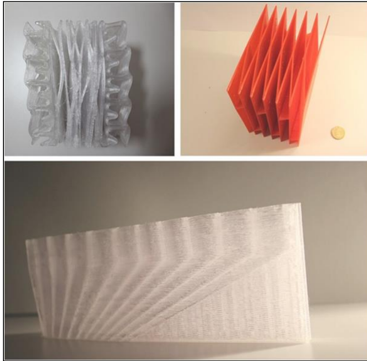
Fig.5. Spong3D: application [15]
